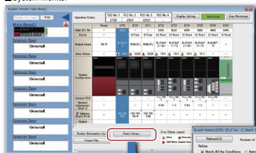
■System Monitor
