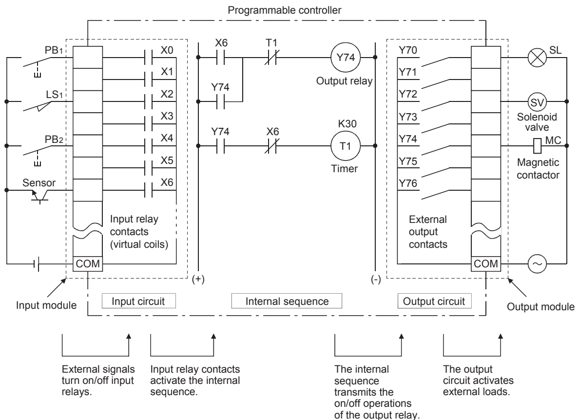
Figure 1.1 Configuration of a programmable controller
